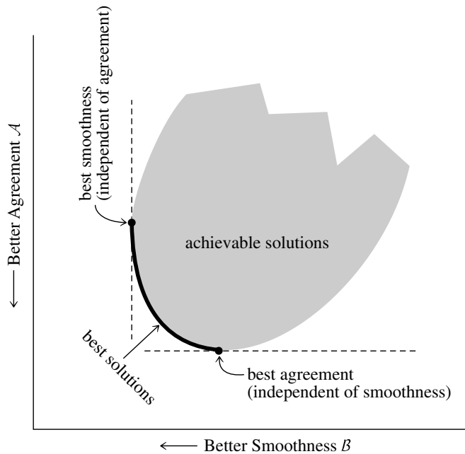
Figure 19.4.1. Almost all inverse problem methods involve a trade-off between two optimizations: agreement between data and solution, or “sharpness” of mapping between true and estimated solutions (here denoted \mathcal{A} ), and smoothness or stability of the solution (here denoted \mathcal{B} ). Among all possible solutions, shown here schematically as the shaded region, those on the boundary connecting the unconstrained minimum of \mathcal{A} and the unconstrained minimum of \mathcal{B} are the “best” solutions, in the sense that every other solution is dominated by at least one solution on the curve.
